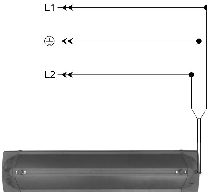
Figure 3.7 • Single Phase Service
