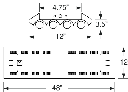
Figure 1.2 • Dual Lamp Fixture Dimensions
