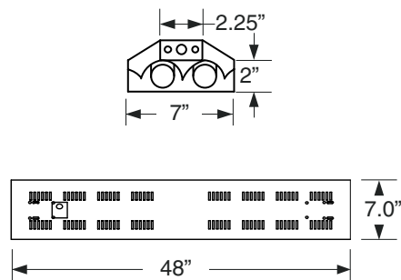
Figure 1.3 • Six Lamp Fixture Dimensions
