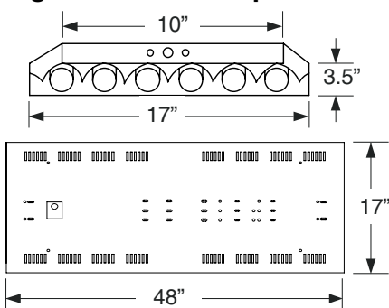
Figure 1.3 • Six Lamp Fixture Dimensions
